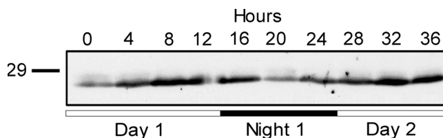
Figure 5 Diurnal changes in At5g39790 protein in spinach leaf. Spinach plants were grown in 12 hour cycle of light and dark and harvested at the times shown. Samples were processed, run on 12% SDS-PAGE, blotted and probed with antibodies generated against At5g39790. The open and solid bars below the blot indicate if samples were taken in the light (open bar) or dark (solid bar). The equivalent of 7.5 mg fresh weight leaf extract was analyzed for each sample.
