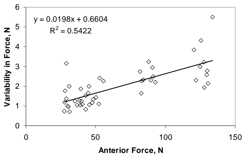
Figure 5-29: Variability in force over 1 minute scan length shows a general increase with anterior force during ascending loading
