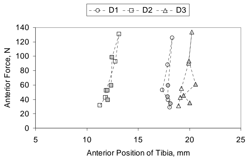
Figure 5-7: KLA Anterior Force-Displacement (S02) showing force ascending (open symbols) and descending (closed symbols) over three test days (D1, D2, D3)
