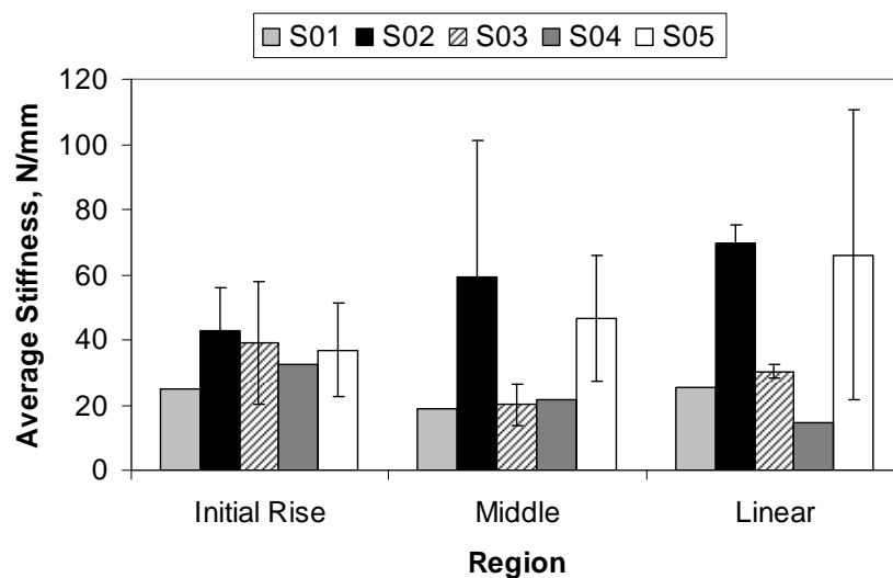
Figure 5-25: KT-2000 average Stiffness for the three regions of the force-displacement curve
