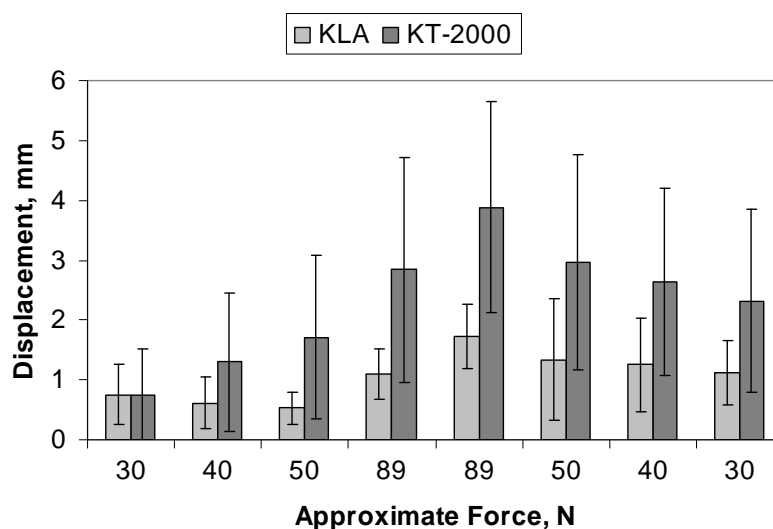
Figure 5-23: Mean displacement at each load level for the KLA and KT-2000 (n=5)
