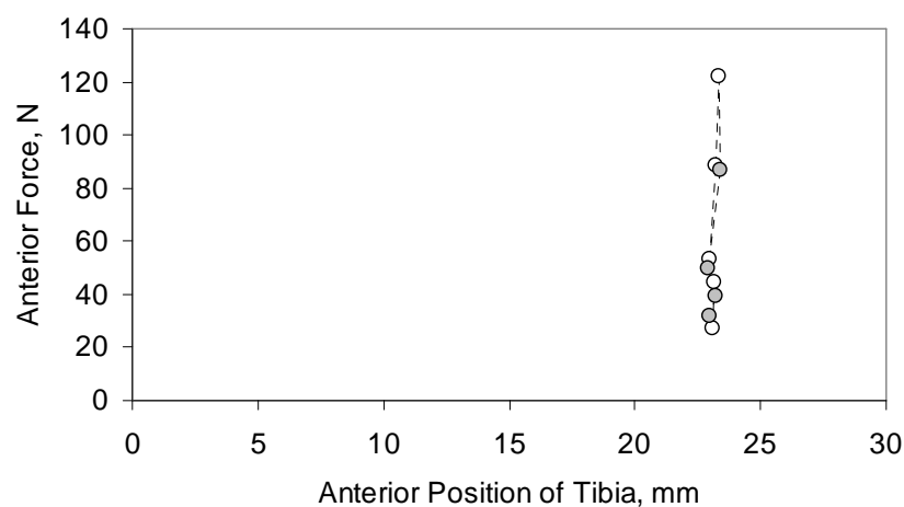
Figure 5-6: KLA Anterior Force-Displacement (S01) showing force ascending (open symbols) and descending (closed symbols)
