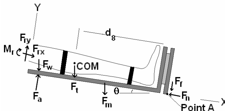
Figure 3-9: Free Body Diagram of the indeterminate force system for the KLA during testing. Forces include the applied force from the hydraulic force system ( F_a ), the reaction forces and moments at the knee ( F_{ry} , F_{rx} , M_r ), the counteractive mass ( F_w ), the KLA mass ( F_m ), and the reaction forces at the hinge ( F_f , F_n ).
