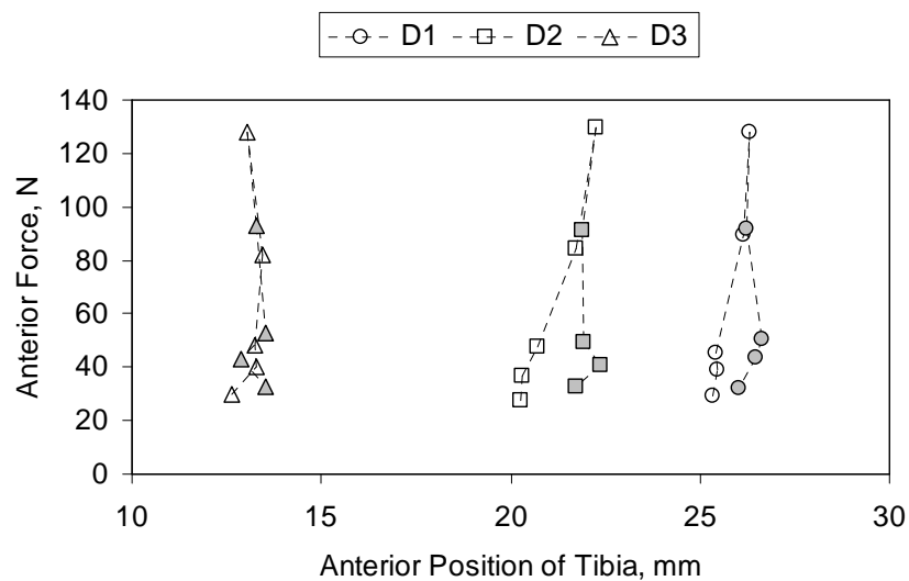
Figure 5-8: KLA Anterior Force-Displacement (S03) showing force ascending (open symbols) and descending (closed symbols) over three test days (D1, D2, D3)
