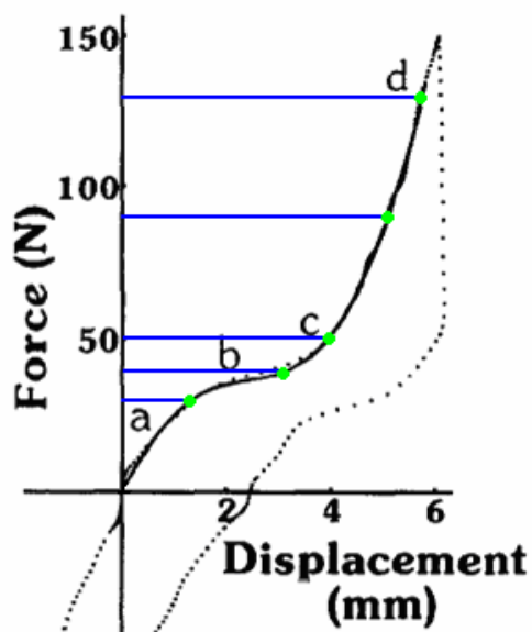
Figure 3-5: Figure 1 from Maitland et al. (1995) showing a representative force-displacement curve from an uninjured subject; modified to show the five load levels chosen to characterize the force-displacement curve. “The initial steep rise in curve is due to the weight of the leg (a). Middle region (b). The inflection point (c) is assumed to be due to the onset of the primary restraints to anterior displacement of the tibia, and by definition results in the x intercept of the second derivative. The cut –off point (d) was chosen at an anterior applied force of 134 N.”
