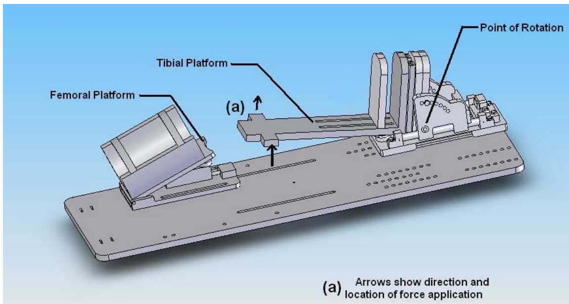
Figure 3-4: 3D Solidworks (Solidworks Corp., Concord, MA, USA) model of the positioning apparatus with force applied at the proximal end of the tibia (a)
