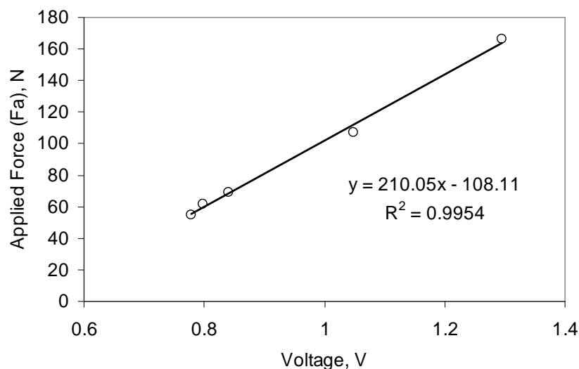
Figure 3-8: Force-Voltage relationship from calibration of KLA
