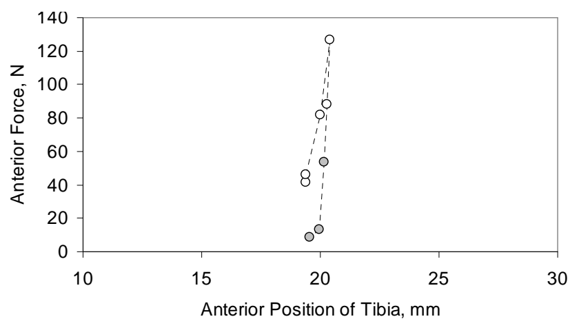
Figure 5-9: KLA Anterior Force-Displacement (S04) showing force ascending (open symbols) and descending (closed symbols)
