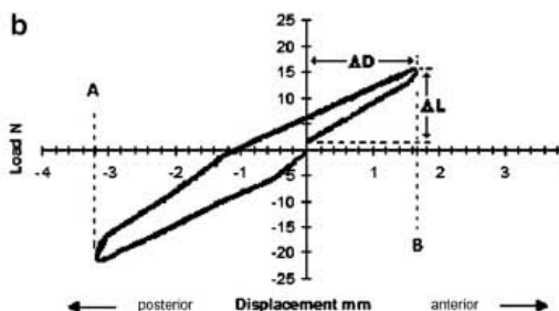
Fig. 1. (a) Positioning of subject for testing with the KT-2000 arthrometer. Modified from "Quadriceps active test at 30^\circ " reprinted with permission from MEDMetric Inc. (b) A typical force–displacement curve resulting from testing with the KT-2000 arthrometer; "A" and "B" denote peak posterior and anterior displacement respectively. The compliance index for the anterior drawer test is calculated as \Delta L/\Delta D .
