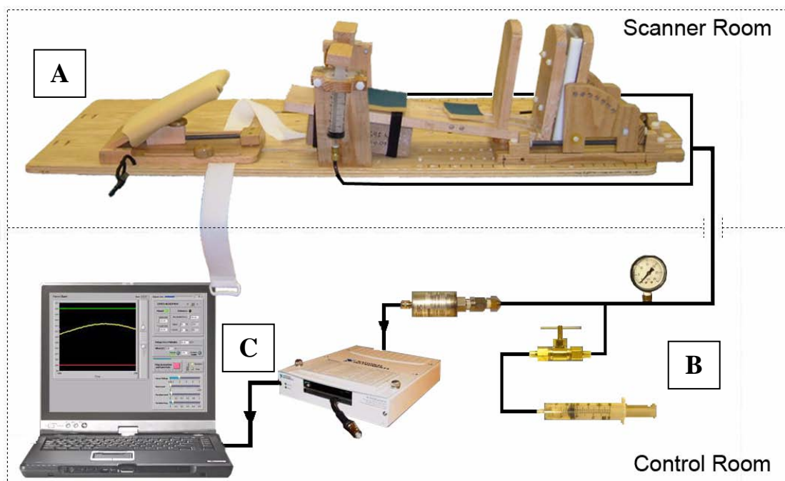
Figure 3-2: KLA System Components including a positioning apparatus [A], hydraulic system [B], and software interface [C]
