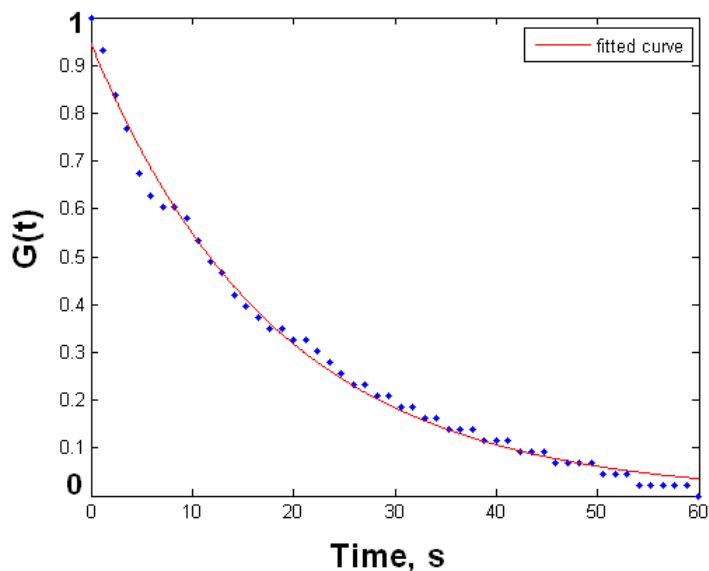
Figure 5-27: Exemplary Stress Relaxation Curve showing G(t) (fitted curve, red) and the raw data (blue)
