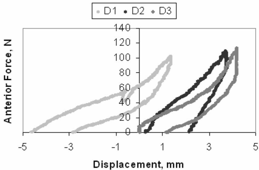
Figure 5-20: KT-2000 Force-Displacement (S03) showing filtered raw data across three days (D1, D2, D3)
