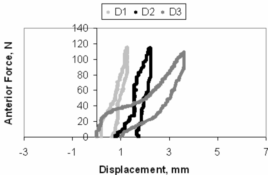
Figure 5-22: KT-2000 Force-Displacement (S05) showing filtered raw data across three days (D1, D2, D3)
