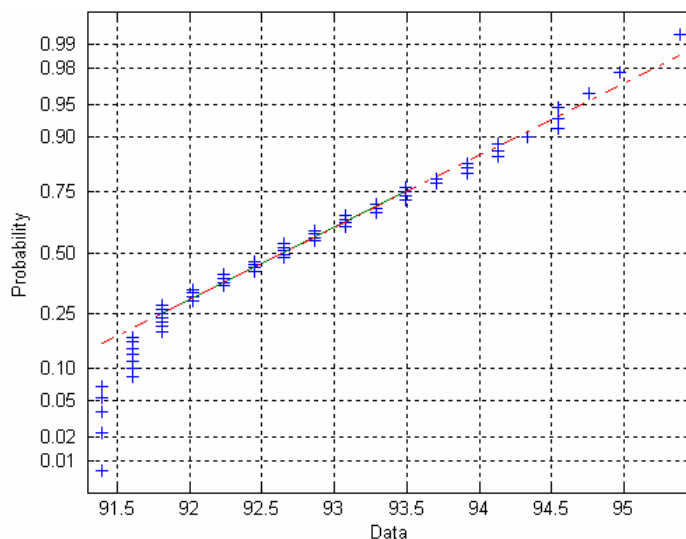
Figure 4-19: Normal Probability Plot for Sample Load Data ( '+' indicates sample data; '--' indicates true normal distribution)
