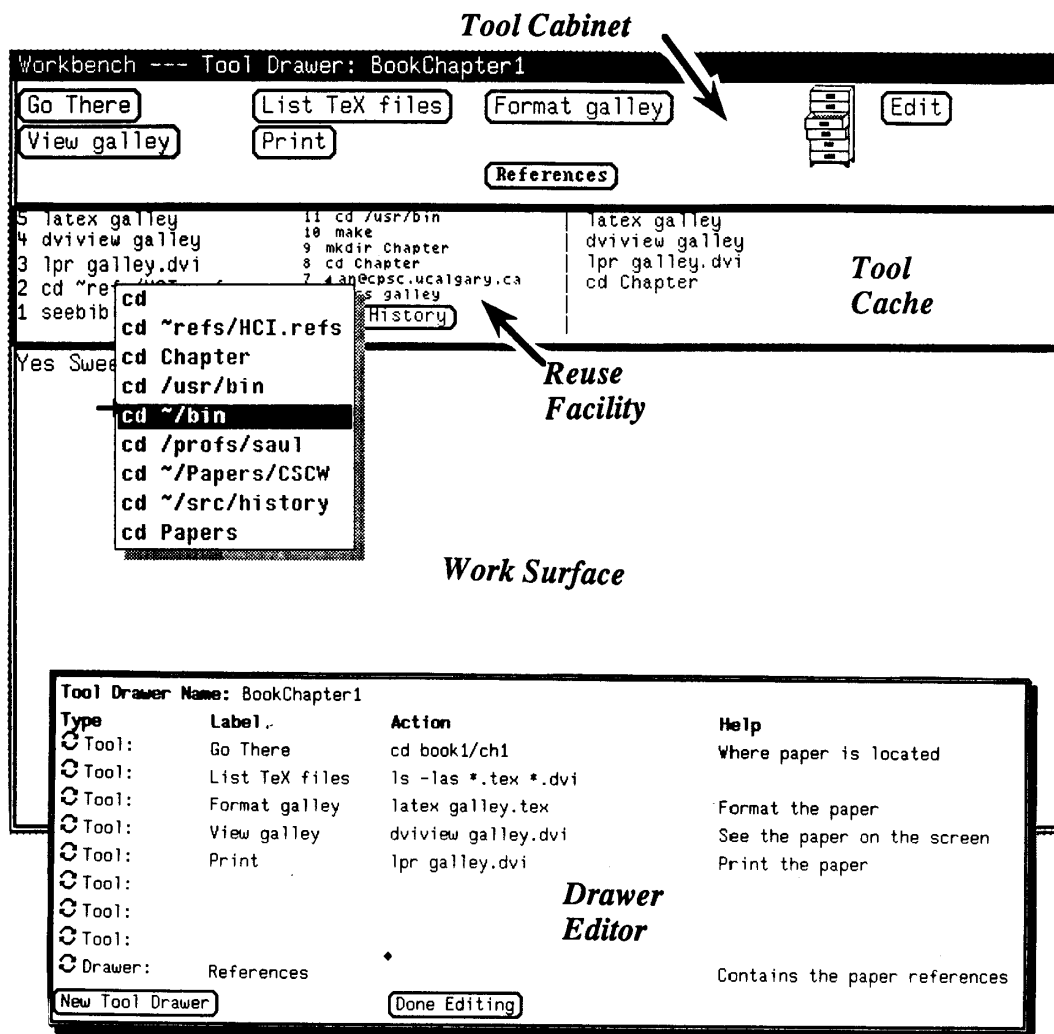
Figure 6: WORKBENCH in use, showing the main WORKBENCH window and two pop up windows
