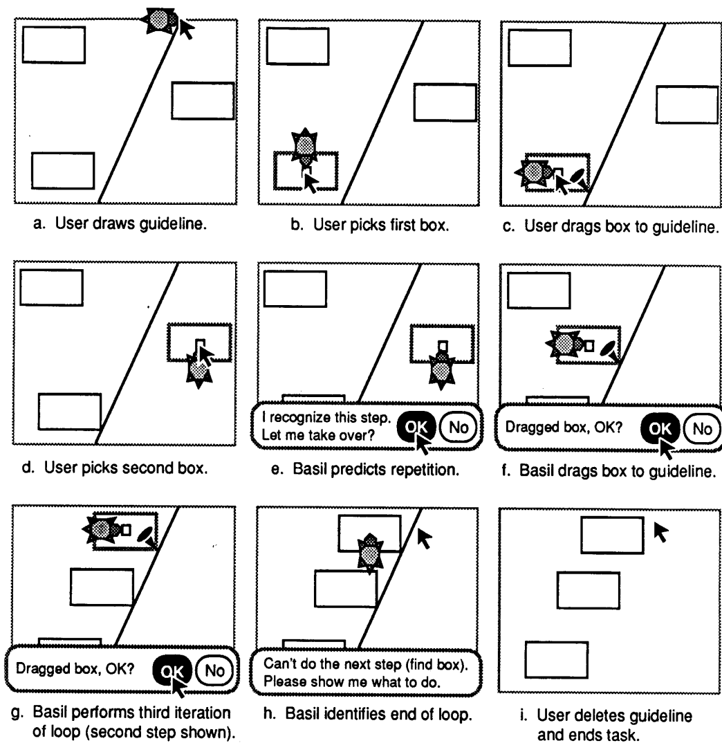
Figure 8: Using Basil to align a set of boxes.
