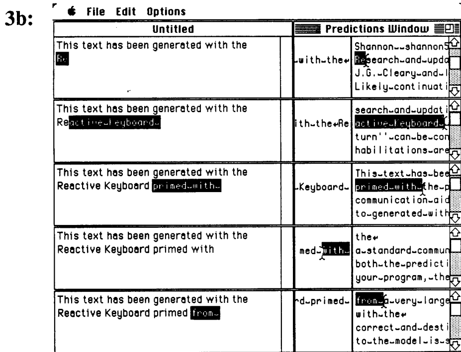
Figure 3. Using RK-pointer, the Macintosh version of the REACTIVE KEYBOARD
