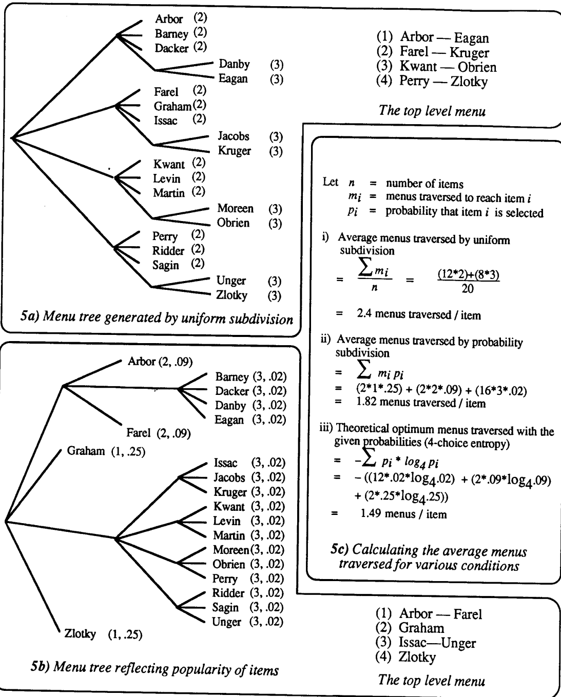
Figure 5: Menu trees generated by uniform and probability subdivision
