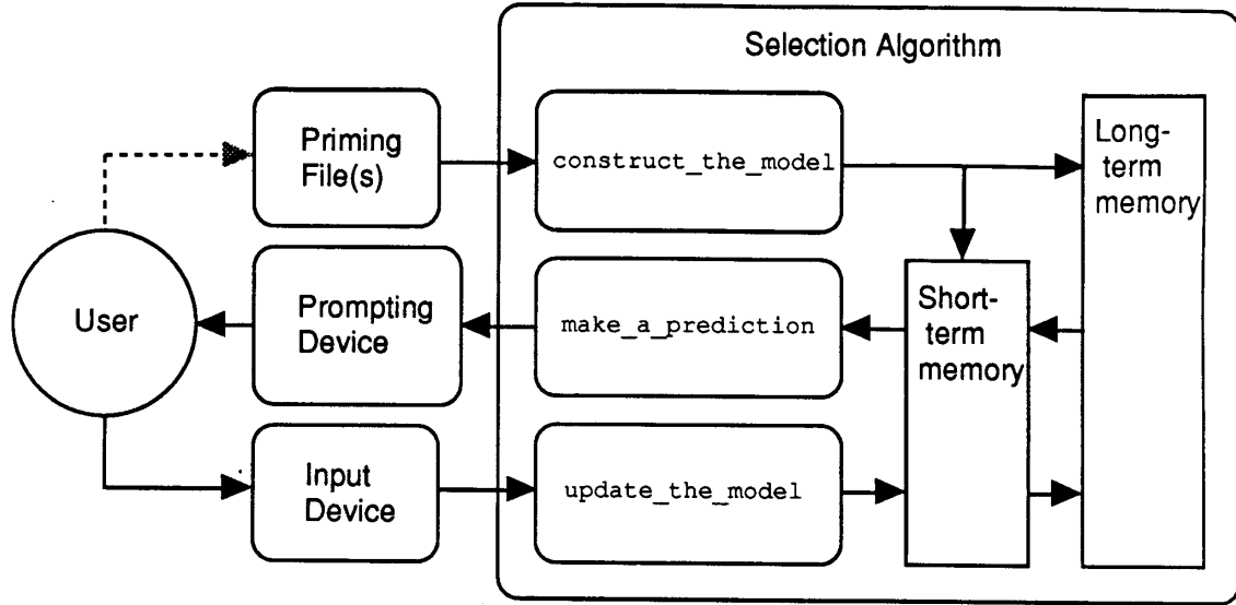
Figure 4: Overview of the REACTIVE KEYBOARD system
