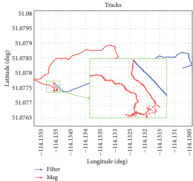
FIGURE 7: Magnetometer heading direction during perturbation area.
