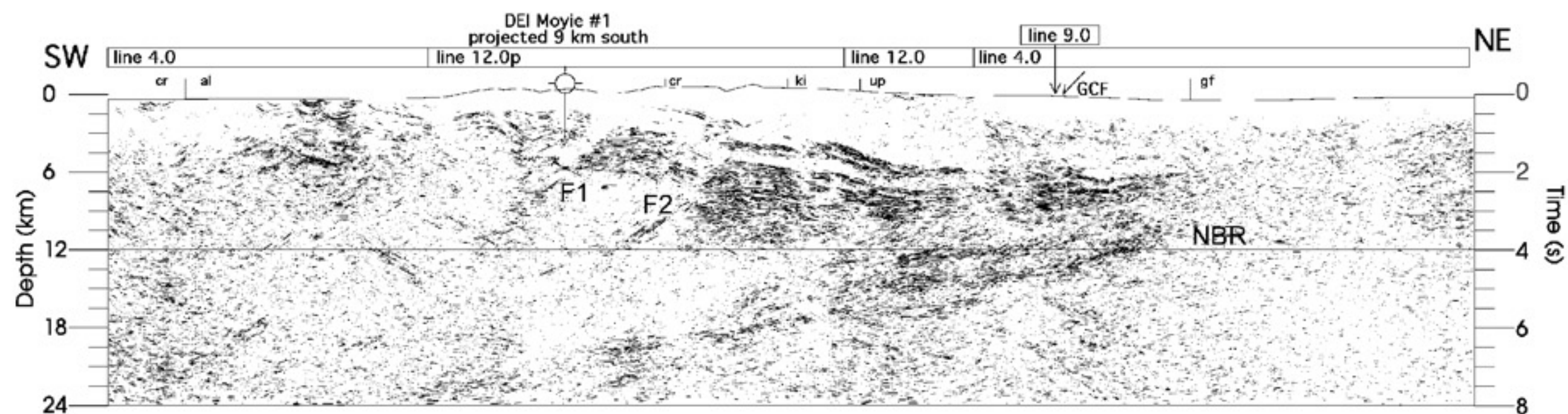
Figure 2-1: Regional data along lines 4.0, 12.0p and 12.0. The geometry of the Moyie sills and near-basement reflectors dominate the structure, though two interpreted faults are also labelled (van der Velden and Cook, 1995).
