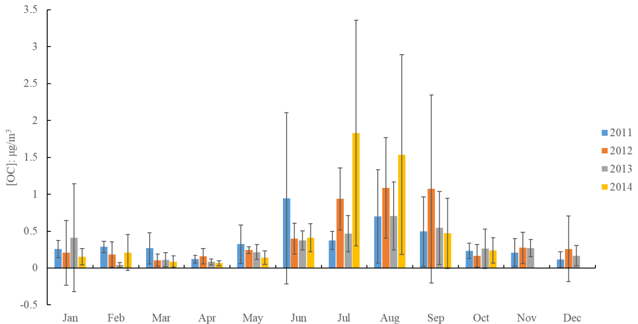
Figure 2-3 Monthly variation of Organic Carbon (OC) for of Barrier Lake 2011-2014 for PM 2.5 .
