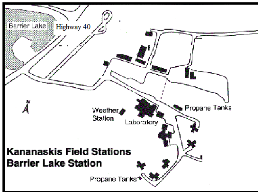
Figure 3-1 Map of Barrier Lake station. (a) A map of Alberta, where Barrier Lake station and the University of Calgary are marked red; (b) A map of locations of the Barrier Lake station and Calgary; (c) Structures at the Barrier Lake station.
