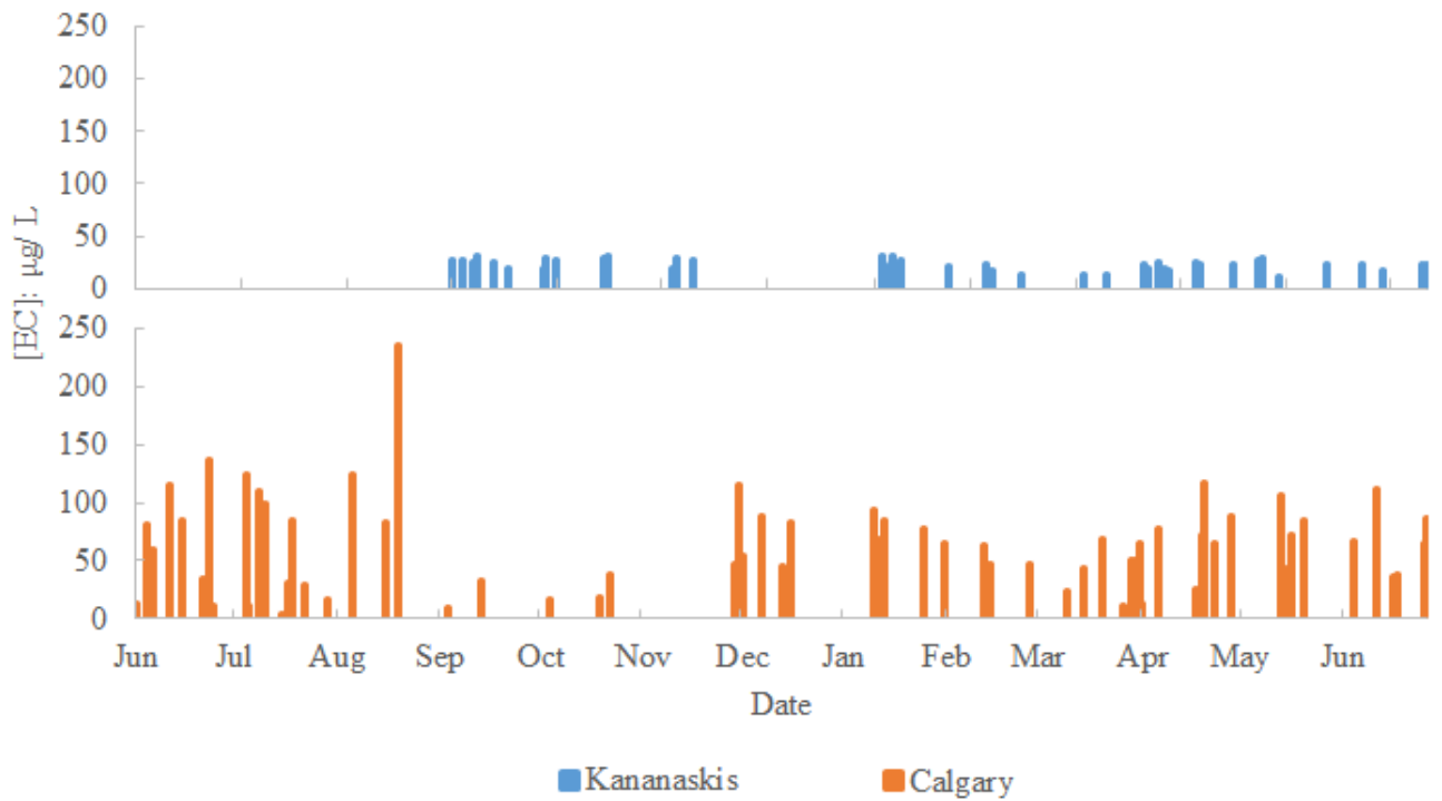
Figure 4-5 Elemental carbon concentration in precipitation samples in Kananaskis and Calgary from June 2016 to July 2017. Note the scale for EC is 32 times lower than that in Figure 4-4.
