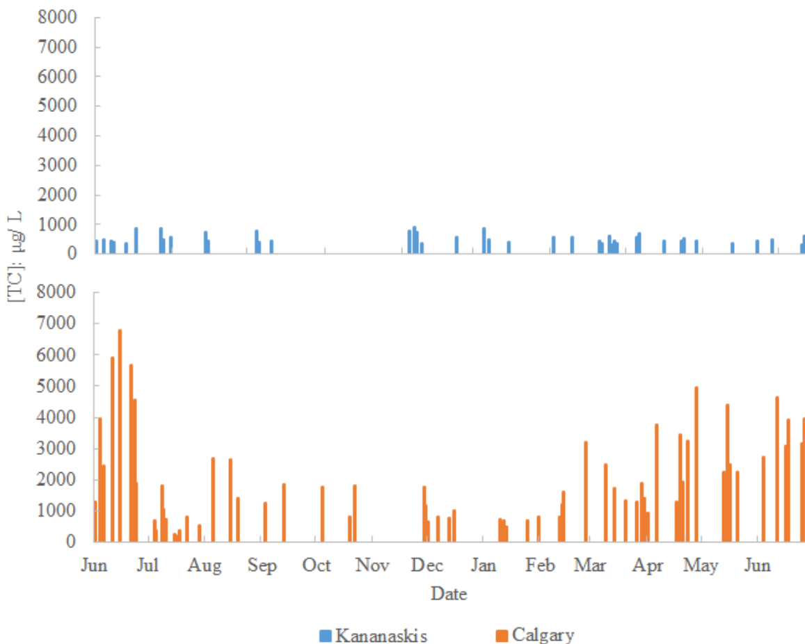
Figure 4-4 Total carbon concentration in precipitation samples.
