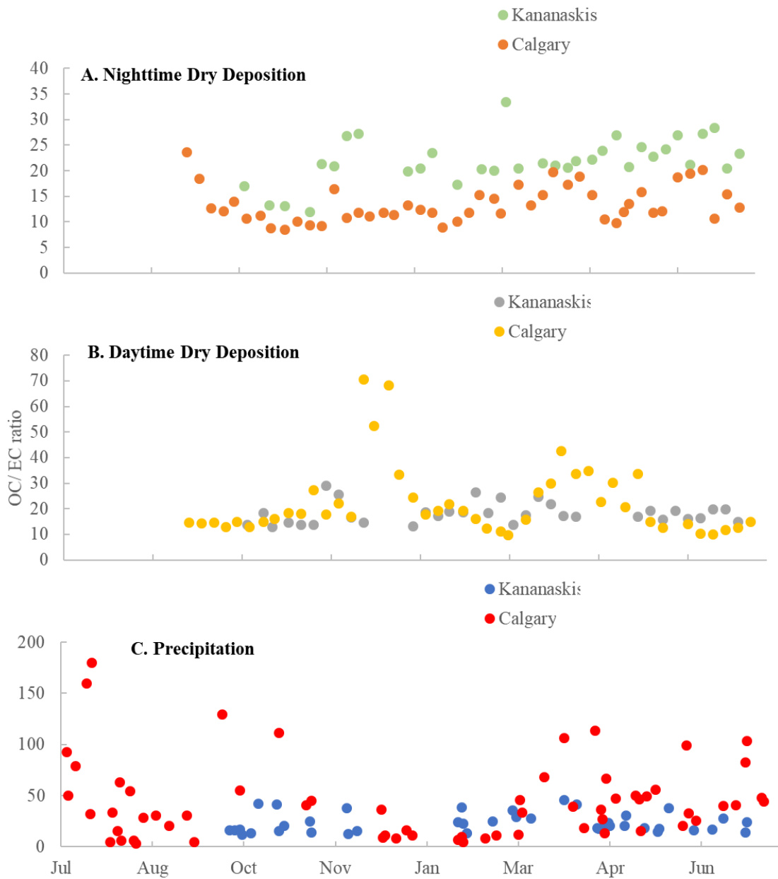
Figure 4-7 OC/EC ratios for all samples collected in Kananaskis and Calgary from July 2016 to June 2017.
