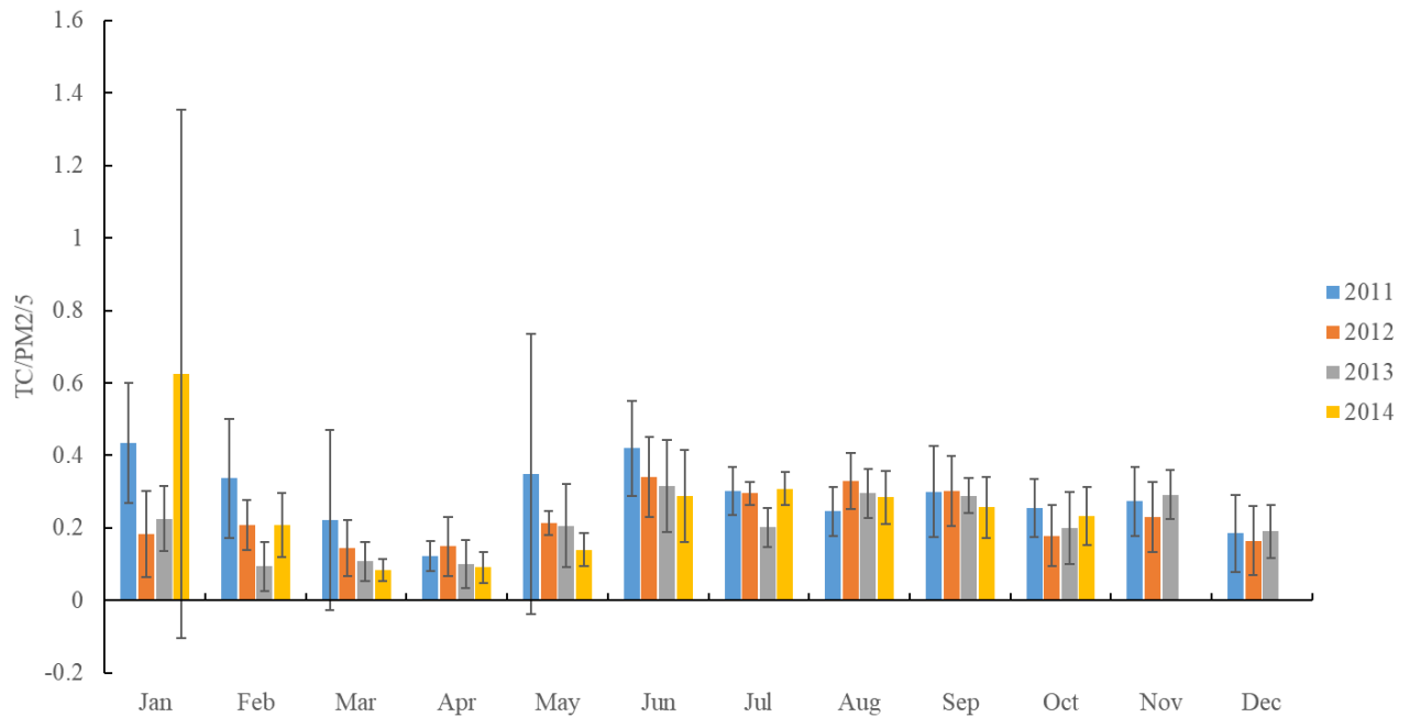
Figure 2-5 Monthly variation of Total Carbon (TC) of Barrier Lake in PM2.5 for 2011-2014.
