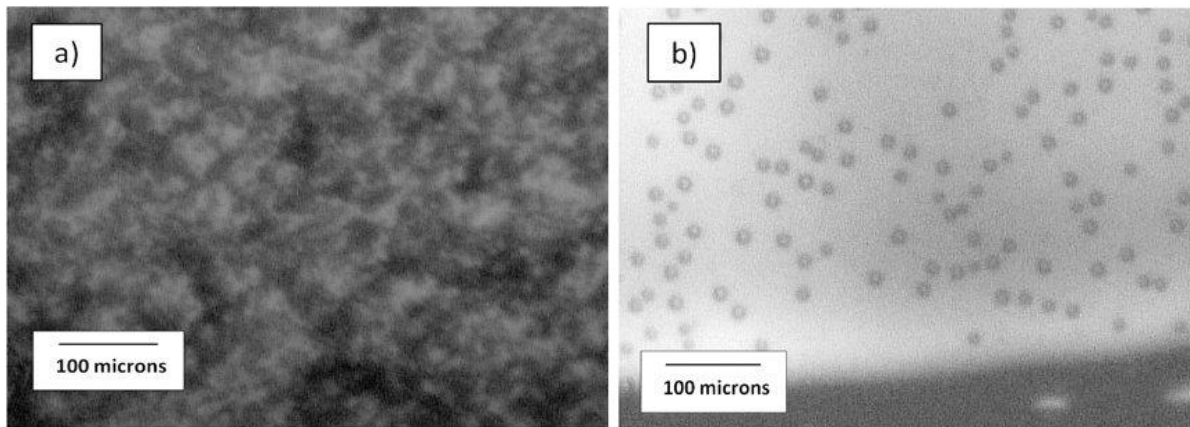
Figure 2.2. Asphaltenes precipitated from bitumen diluted with n-pentane, images captured by HPM: a) 23°C (glassy particles); b) 165°C (liquid droplets) (Johnston et al. , 2017).
