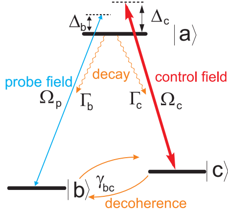
Figure 3.1: A \Lambda -type atom with associated coupling fields and decoherence and decay mechanisms shown. Rubidium atoms, which will be utilized in this work, exhibit this type of energy level scheme.
