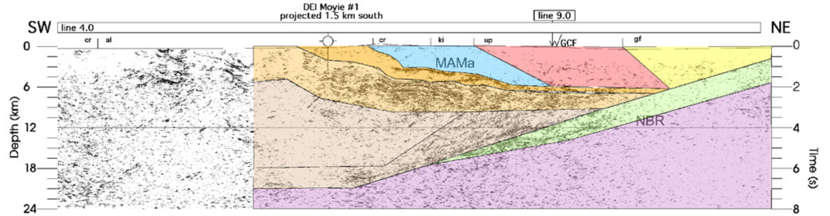
Figure 4-3: Duncan line 4.0 with an interpretation overlain on the portion of line that runs approximately east-west. This was used in building the model for profile 4. The Duncan Energy exploration well is labelled.
